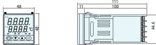
External Dimensions
